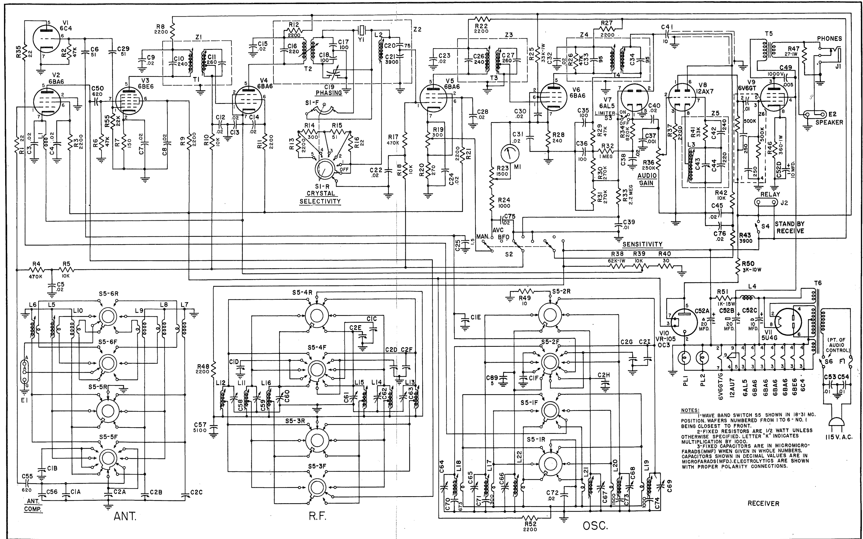
Figure 7. Hammarlund HQ-140XA, Schematic Diagram
